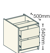
▲ Bedside 2 Drawer Unit* 2 Drawers (215mm high)
