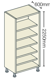
▲ Fully Shelved Robe 5 Shelves
