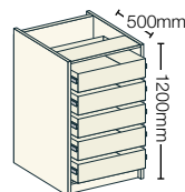
▲ Tall 5 Drawer Unit*** 5 Drawers (215mm high)
