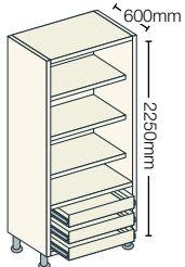
▲ Fully Shelved Combi Robe with 3 External Drawers 3 Shelves 3 External Drawers
