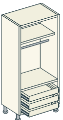
▲ Combi Robe with 3 External Drawers 1 Hanging Rail 1 Shelf
