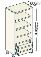
▲ Combi Robe with 3 Shelves & 3 Internal Drawers 3 Shelves 3 Internal Drawers
