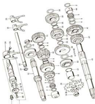
8. Transmission Gears 1/2
