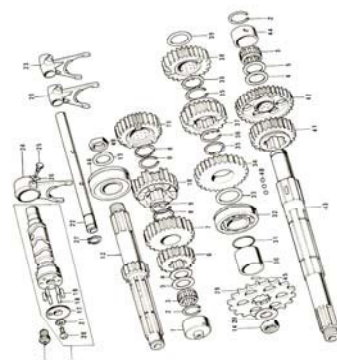
8. Transmission Gears 2/2
