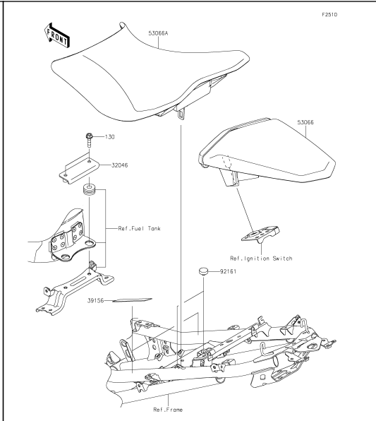
50 Seat
