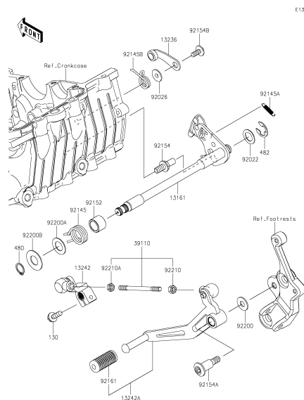
13 Gear Change Mechanism
