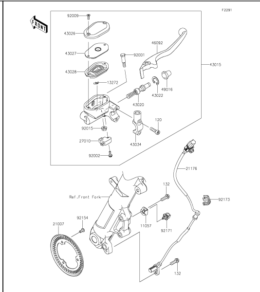
43 Front Master Cylinder
