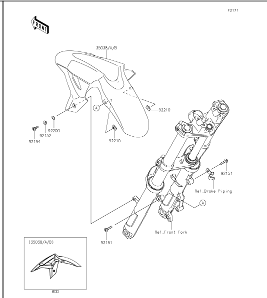
35 Front Fender(s)
