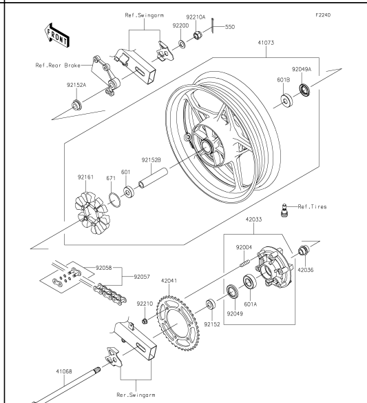
40 Rear Hub
