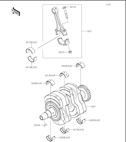
8 Crankshaft
