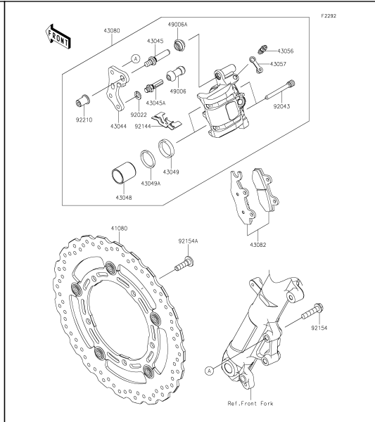
44 Front Brake
