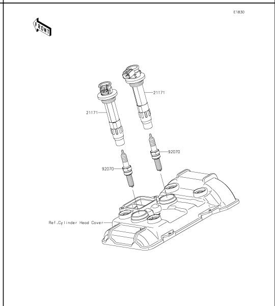
24 Ignition System
