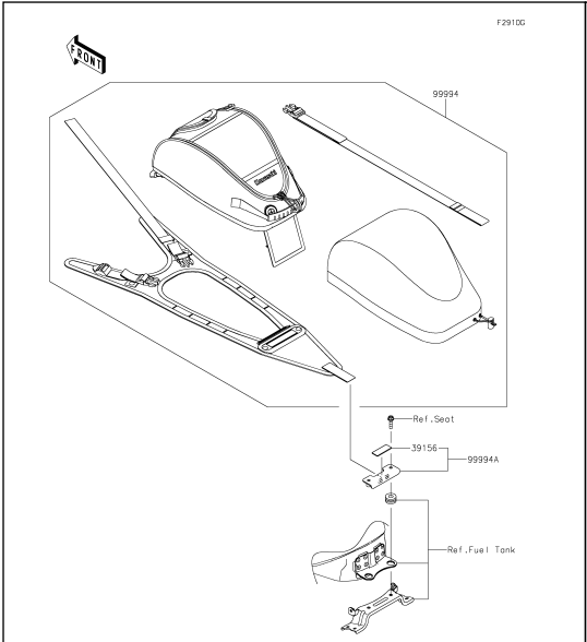
73 Accessory(Tank Bag)
