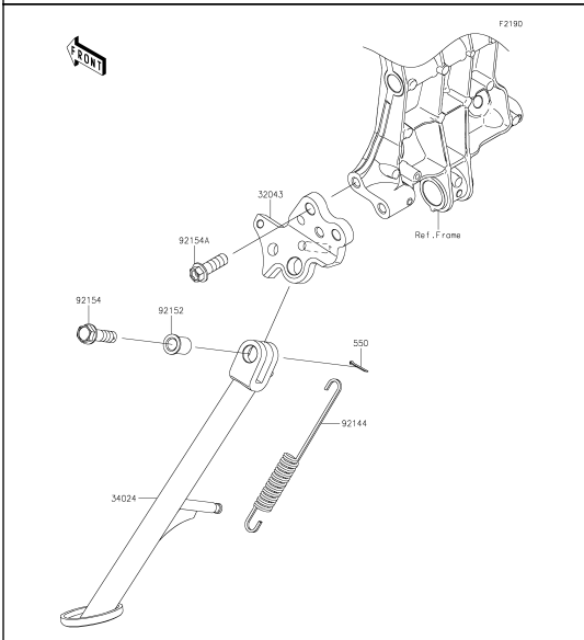
37 Stand(s)
