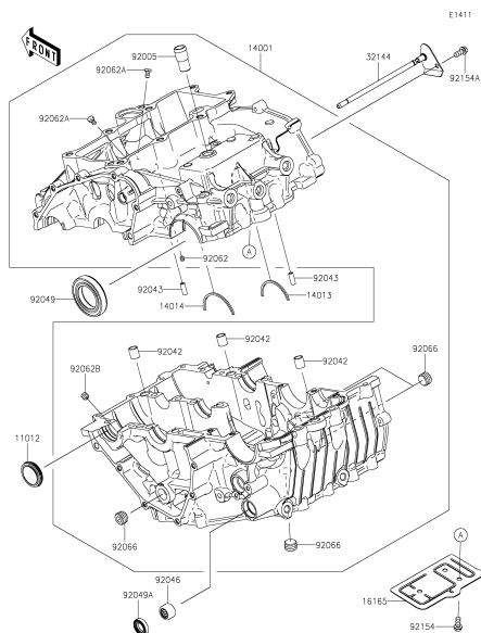
14 Crankcase
