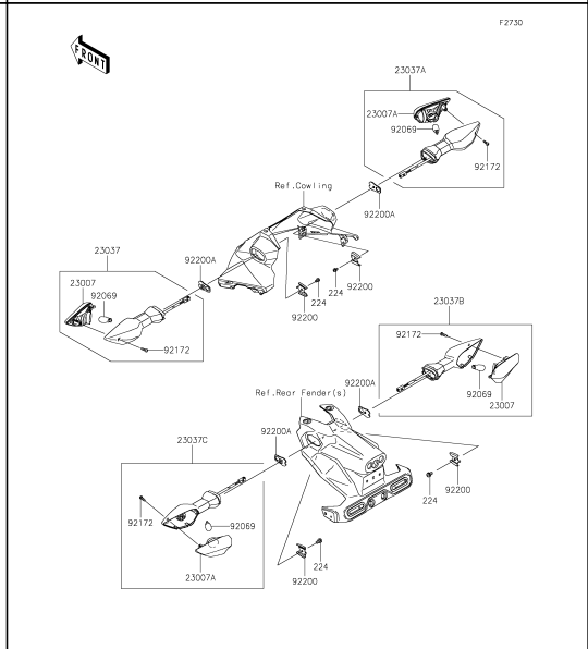
56 Turn Signals
