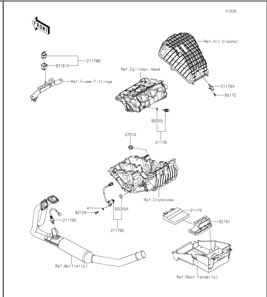
20 Fuel Injection
