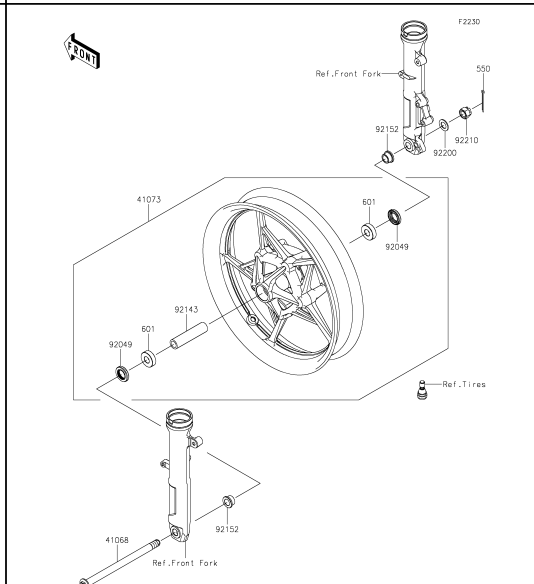
39 Front Hub
