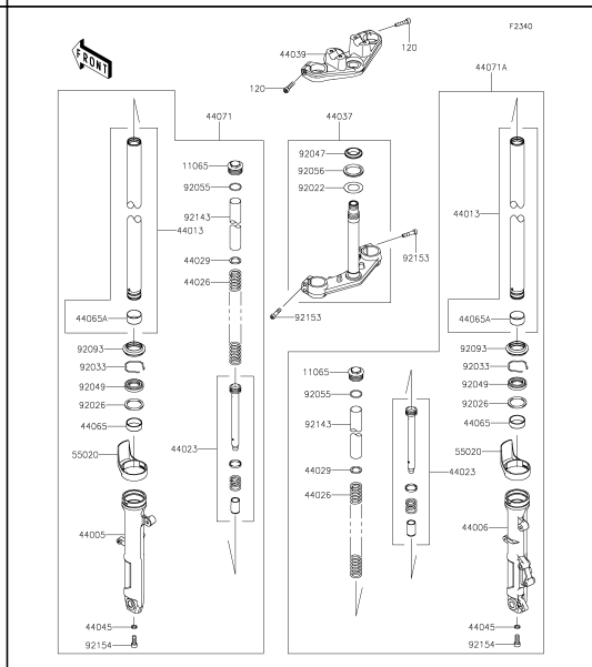
48 Front Fork
