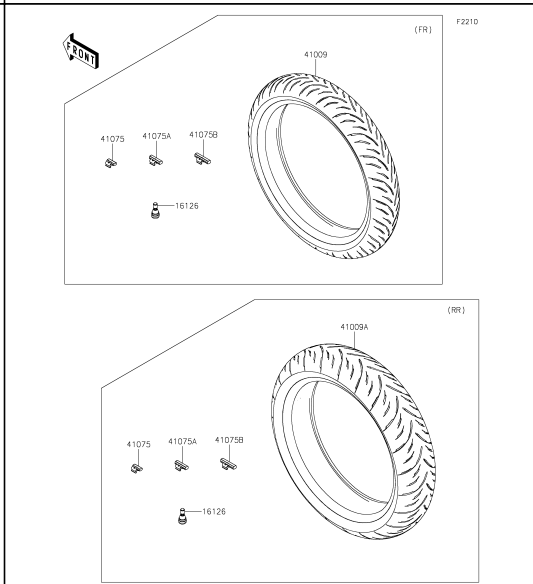
38 Tires
