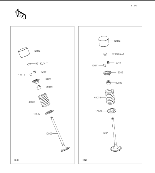
6 Valve(s)
