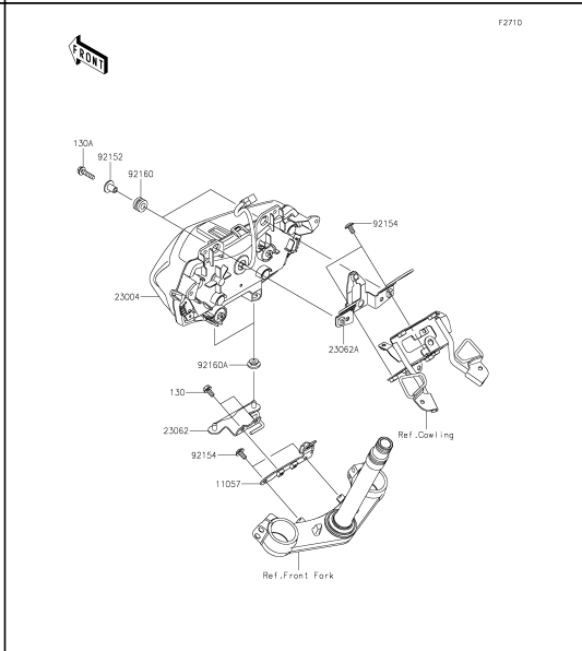
54 Headlight(s)
