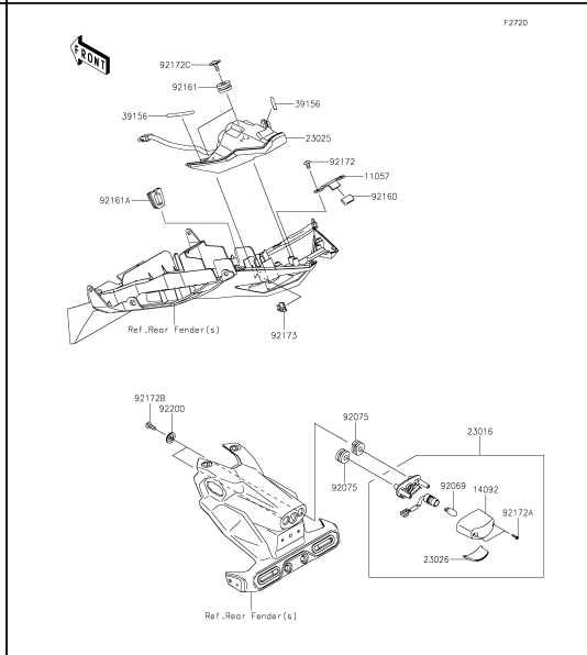
55 Taillight(s)
