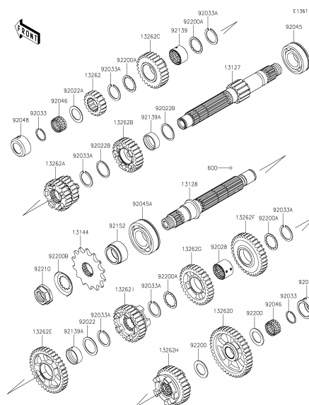
11 Transmission
