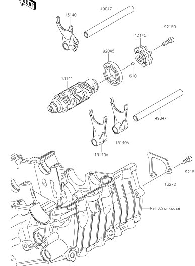
12 Gear Change Drum/Shift Fork(s)
