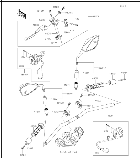
47 Handlebar
