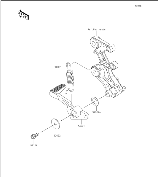
41 Brake Pedal
