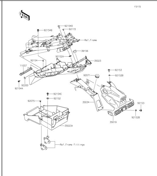
36 Rear Fender(s)
