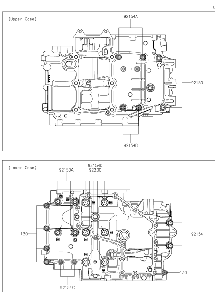
15 Crankcase Bolt Pattern
