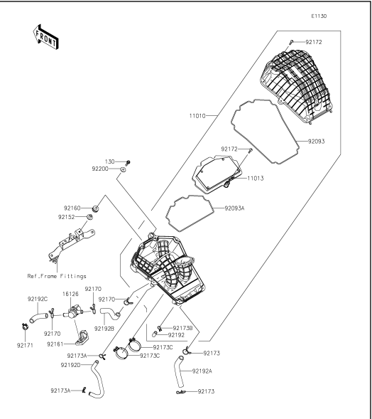
4 Air Cleaner
