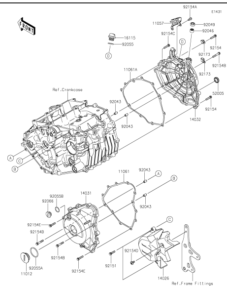
16 Engine Cover(s)
