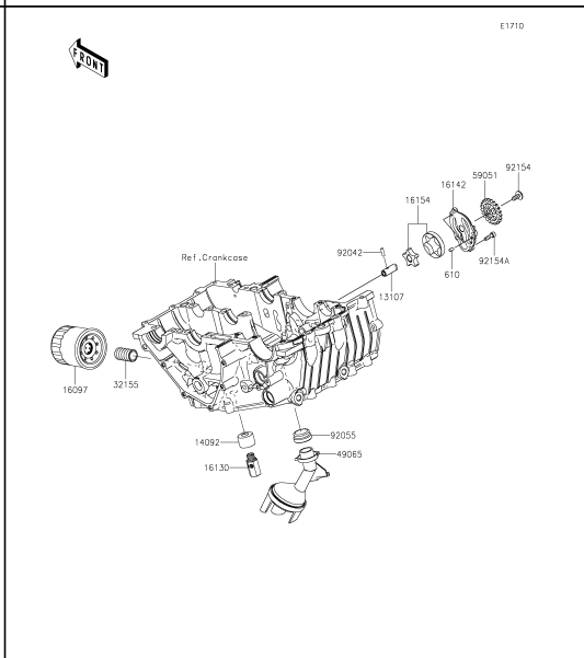
22 Oil Pump
