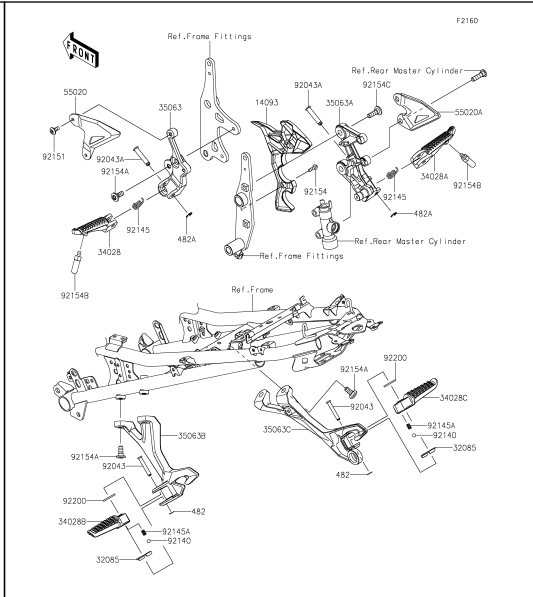
34 Footrests
