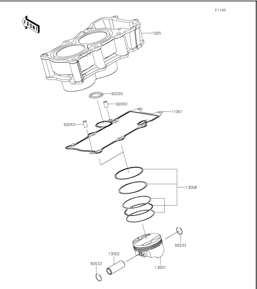
3 Cylinder/Piston(s)
