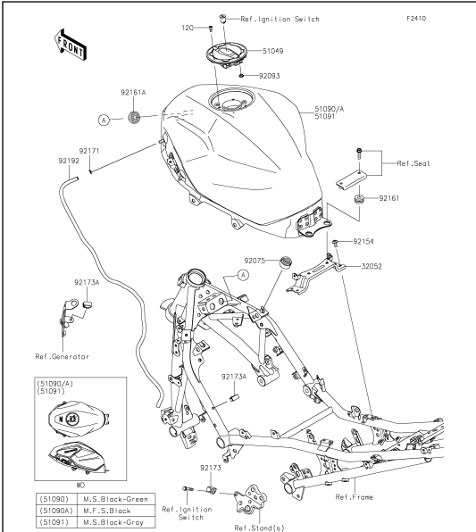
49 Fuel Tank
