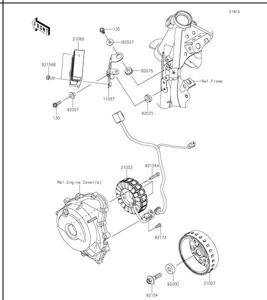
23 Generator
