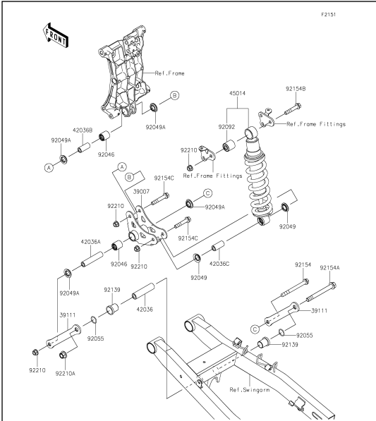
33 Suspension/Shock Absorber
