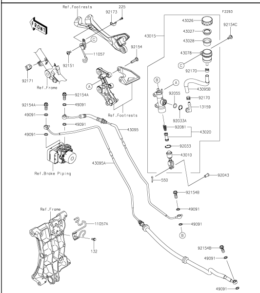
45 Rear Master Cylinder
