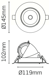
Cut out: Ø120-130mm
