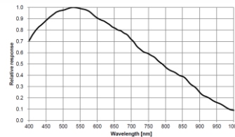
MV-CB060-10UM-S
