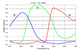
MV-CB060-10UC-S
