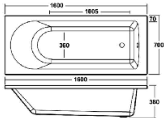
BARMBY 1600x700mm BATH
