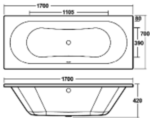
OTLEY 1700x700mm BATH
