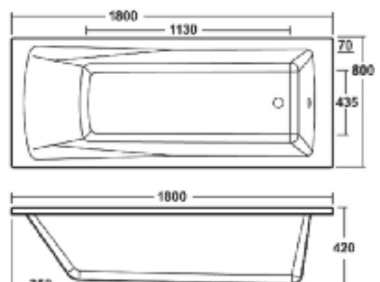
LINTON 1800x800mm BATH
