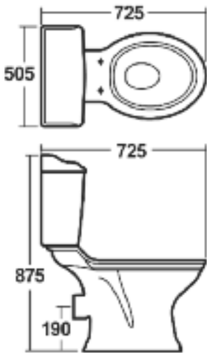
CLOSE COUPLED PAN & CISTERN
