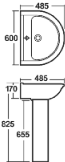
600MM BASIN & PEDESTAL
