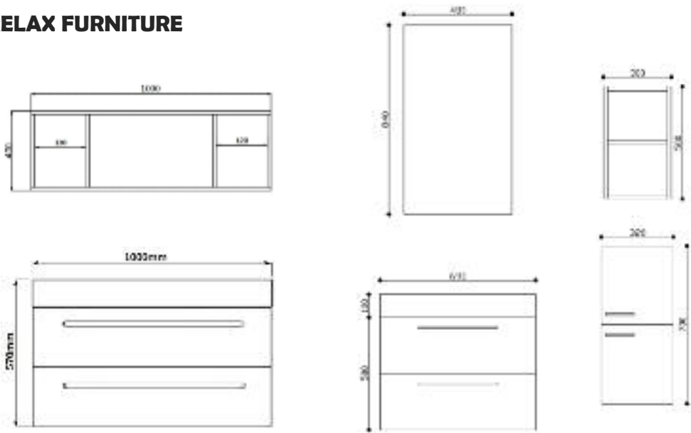
FRE005 - RELAX FURNITURE - BLACK WOOD
