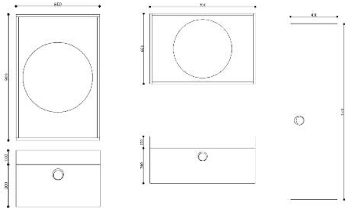
FSO001 SONAR FURNITURE - 600MM
