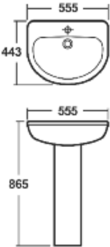
555MM BASIN & PEDESTAL
