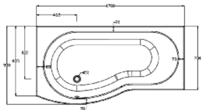
BMP1785L CURVED SHOWER BATH
