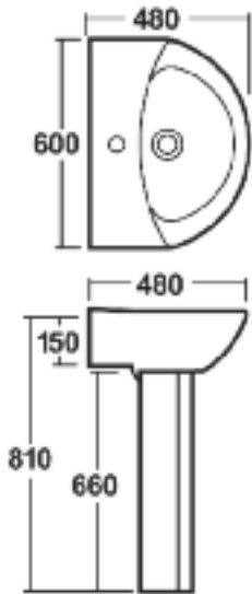
600MM BASIN & PEDESTAL
