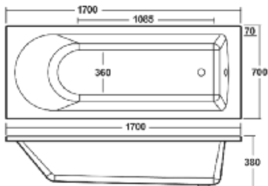
BARMBY 1700x700mm BATH
