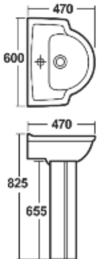
600MM BASIN & PEDESTAL
