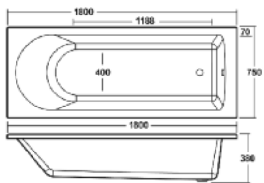
BARMBY 1800x750mm BATH
