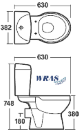
CLOSE COUPLED PAN & CISTERN
