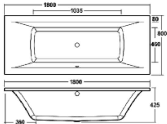
ASSELBY 1800x800mm BATH
