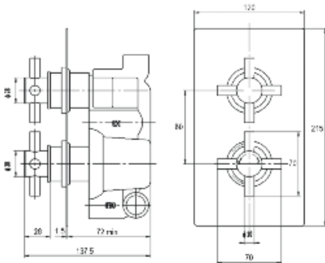
TWIN VALVE - RECTANGULAR PLATE
