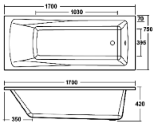
LINTON 1700x750mm BATH
