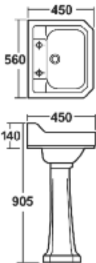
560MM BASIN & PEDESTAL
