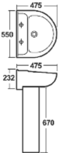
550MM 2TH BASIN & PEDESTAL
