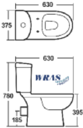
CLOSE COUPLED PAN & CISTERN
