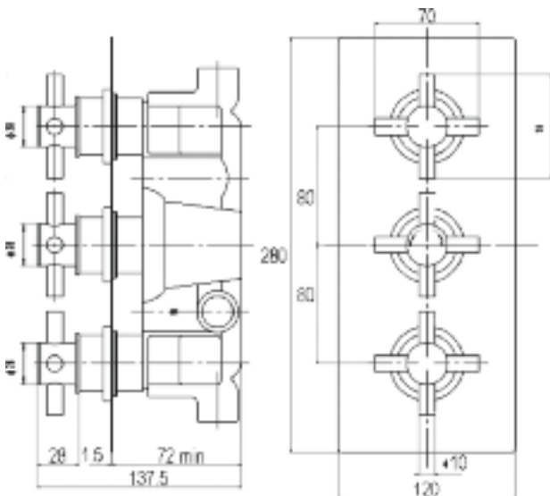
TRIPLE VALVE - RECTANGULAR PLATE
