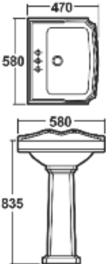
580MM BASIN & PEDESTAL
