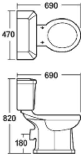
CLOSE COUPLED PAN & CISTERN
