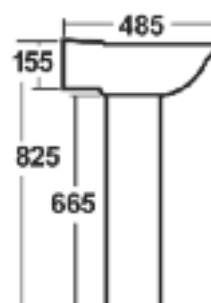
600MM BASIN &amp; PEDESTAL
