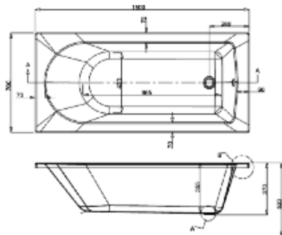
BARMBY 1500x700mm BATH
