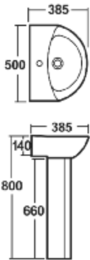
500MM BASIN & PEDESTAL
