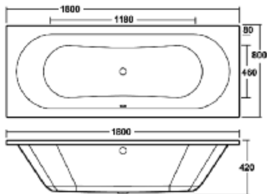
OTLEY 1800x800mm BATH
