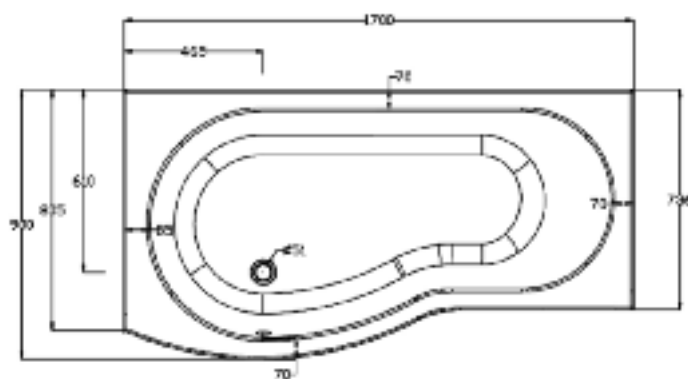
BMP1785R CURVED SHOWER BATH
