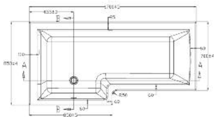
BMBS1785L SQUARE SHOWER BATH
