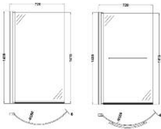
NCS1-NCSO-NCSR1 CURVED BATH SCREENS
