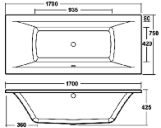
ASSELBY 1700x750mm BATH
