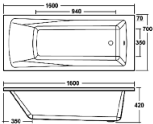
LINTON 1600x700mm BATH
