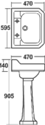
600MM BASIN & PEDESTAL
