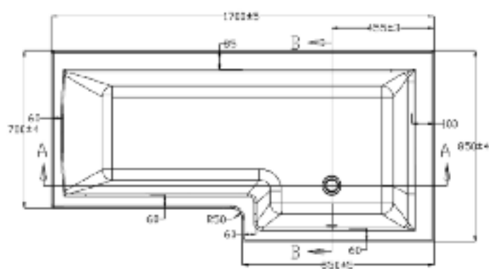
BMBS1785R SQUARE SHOWER BATH
