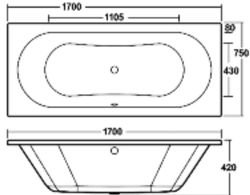
OTLEY 1700x750mm BATH
