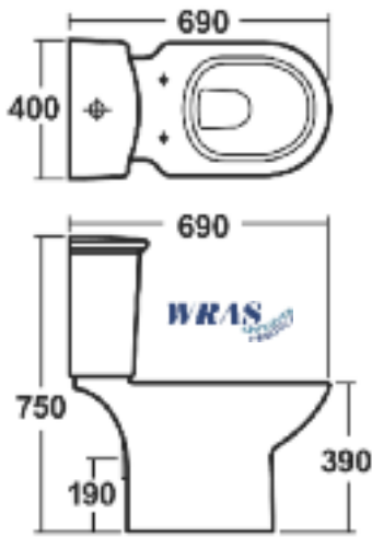
CLOSE COUPLED PAN & CISTERN
