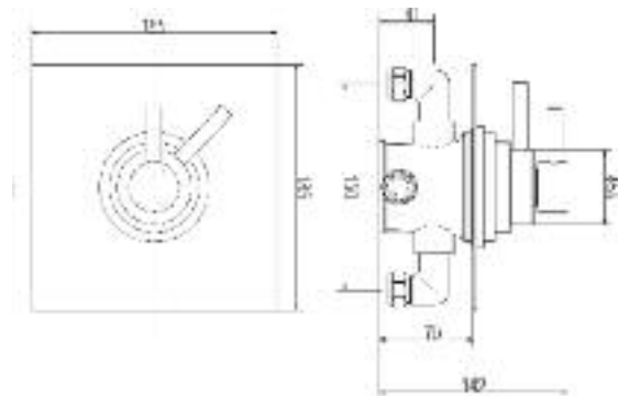
DUAL EXPOSED VALVE
