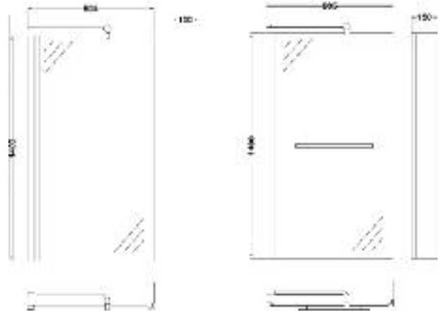
NSB52-NSB5R2 QUATTRO SQUARE BATH SCREENS
