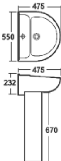
550MM 1TH BASIN & PEDESTAL
