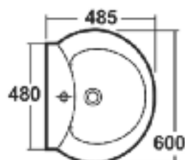
600MM BASIN &amp; PEDESTAL
