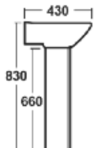
600MM BASIN &amp; PEDESTAL
