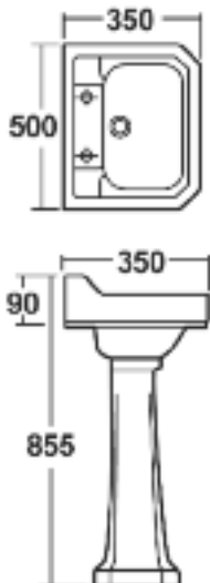
500MM BASIN & PEDESTAL
