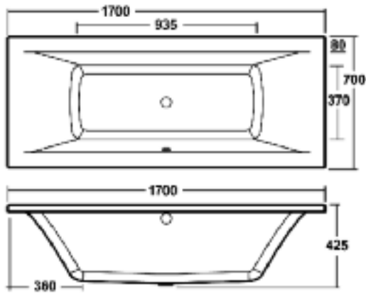
ASSELBY 1700x700mm BATH
