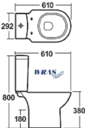
CLOSE COUPLED PAN & CISTERN
