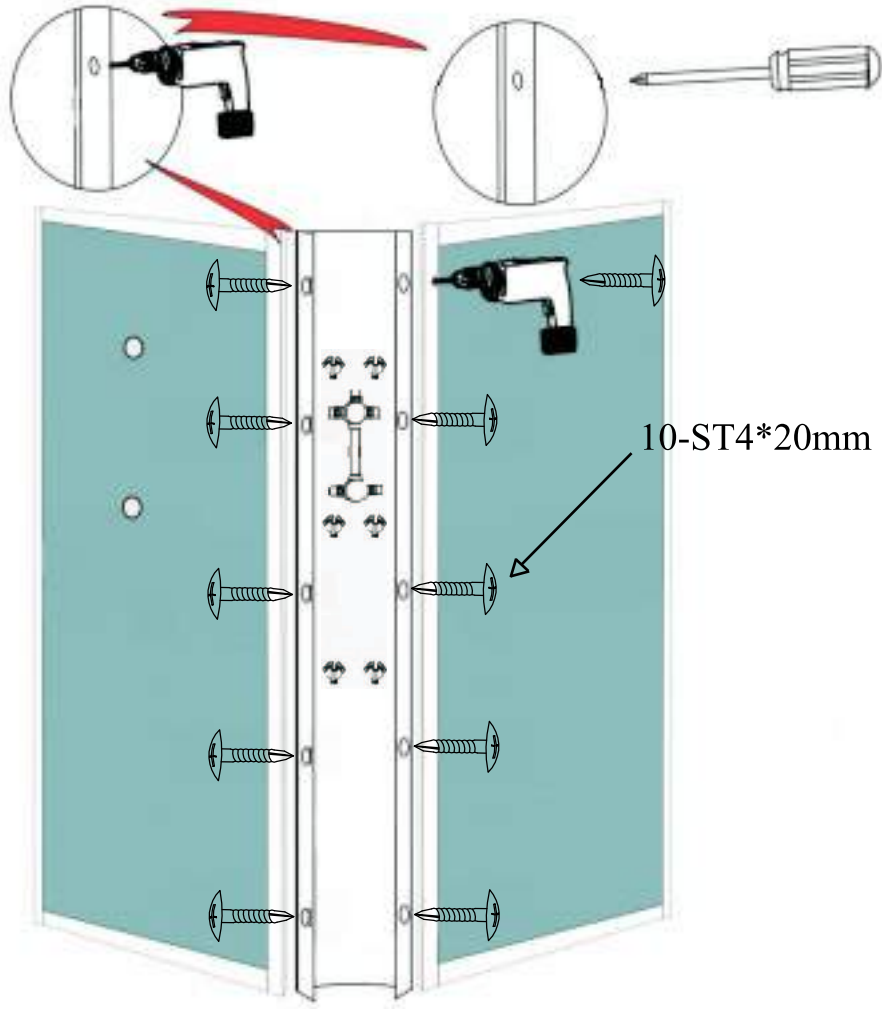
tapping screw
