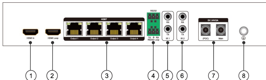
Rear Panel
