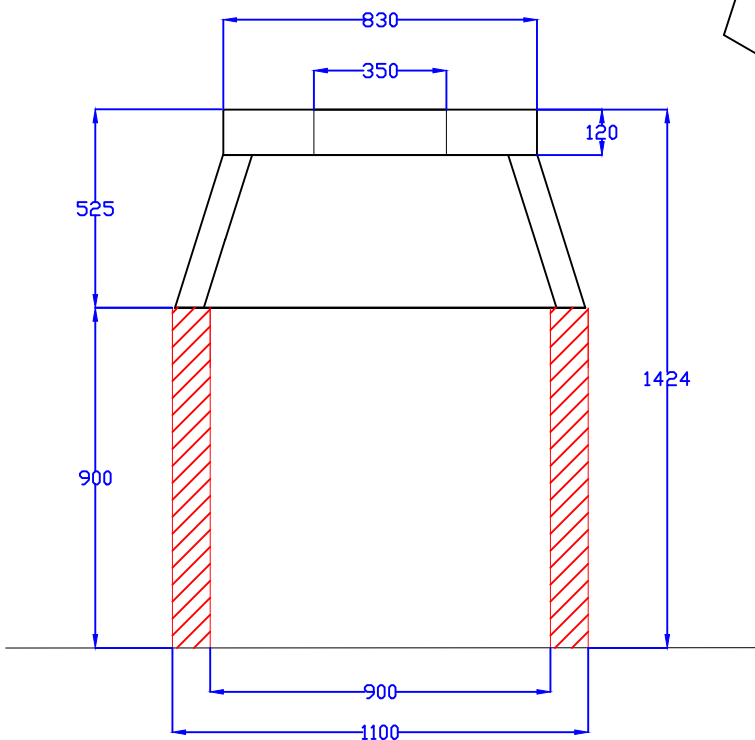
Front Section
