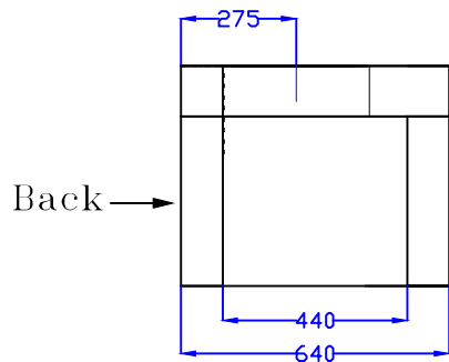
Side Section
