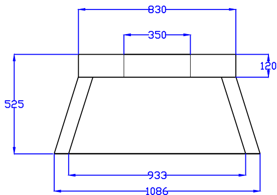
Front Section
