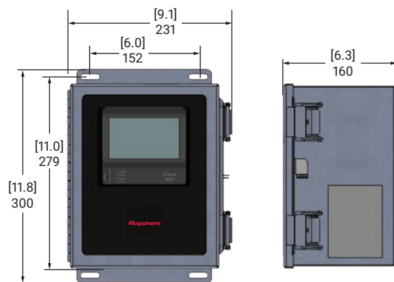
Stainless Steel Enclosure with EMR
