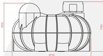
SIDE ELEVATION
