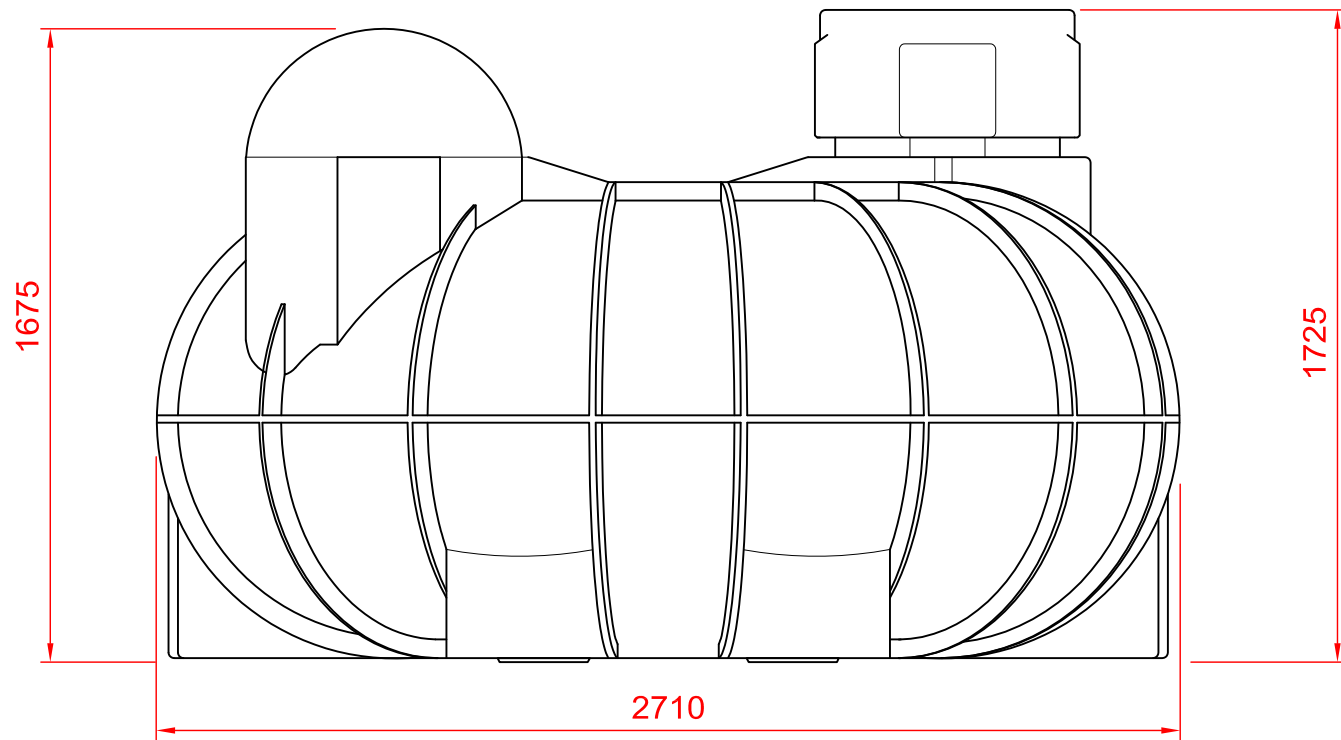
SIDE ELEVATION
