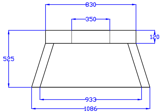
Front Section
