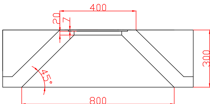
FRONT SECTION
