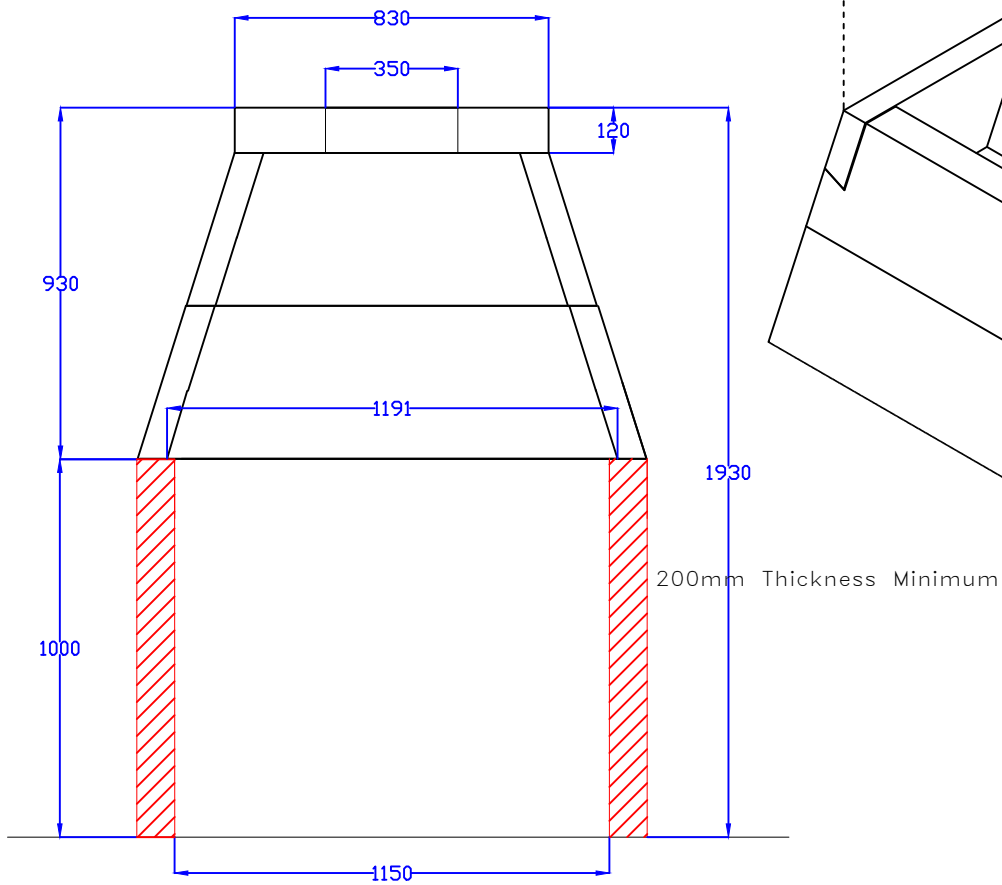
Front Section
