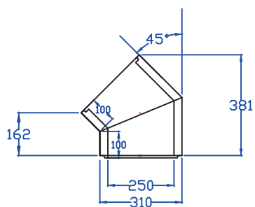
250mm I/D 45DEG BENDS
