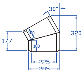
225mm I/D 30DEG BENDS
