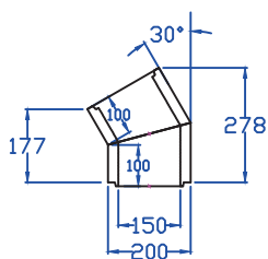
150mm I/D 30DEG BENDS
