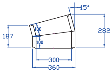
300mm I/D 15DEG BENDS
