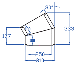
250mm I/D 30DEG BENDS
