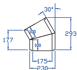
175mm I/D 30DEG BENDS
