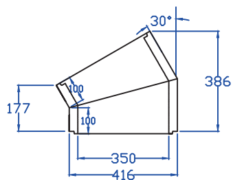
350mm I/D 30DEG BENDS
