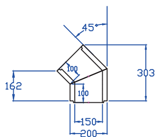
150mm I/D 45DEG BENDS
