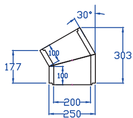
200mm I/D 30DEG BENDS
