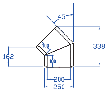
200mm I/D 45DEG BENDS
