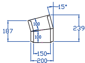
150mm I/D 15DEG BENDS
