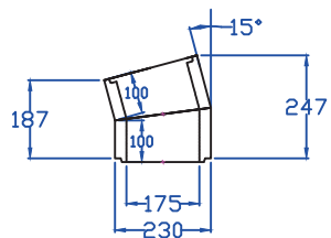
175mm I/D 15DEG BENDS
