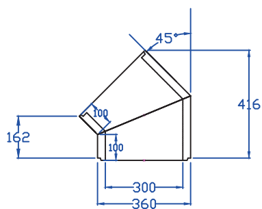
300mm I/D 45DEG BENDS
