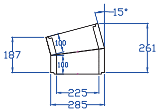
225mm I/D 15DEG BENDS
