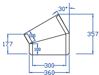
300mm I/D 30DEG BENDS
