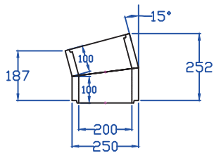
200mm I/D 15DEG BENDS
