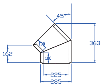
225mm I/D 45DEG BENDS
