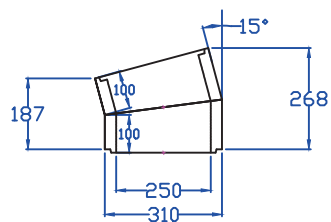
250mm I/D 15DEG BENDS
