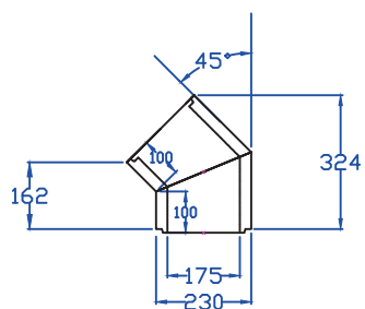
175mm I/D 45DEG BENDS
