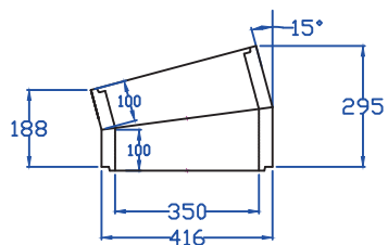
350mm I/D 15DEG BENDS
