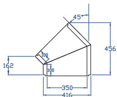
350mm I/D 45DEG BENDS
