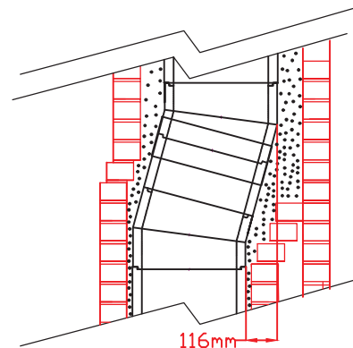
OPTIONAL BACK OFFSET IN LOFT
