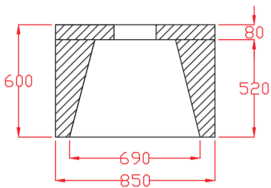
FRONT SECTION OF GATHER
