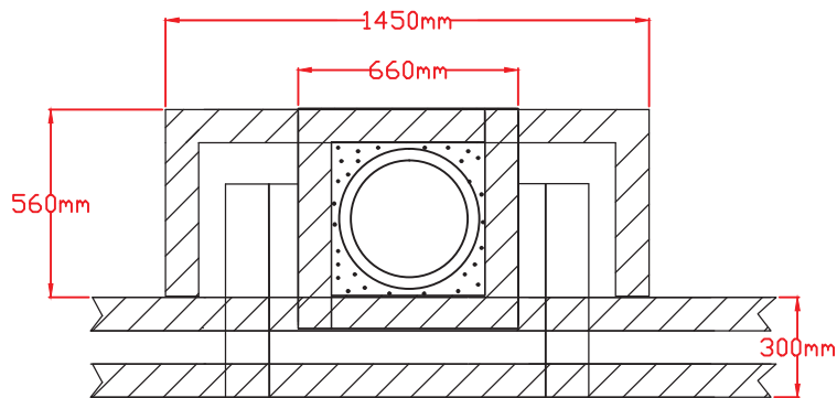
PLAN OF CHIMNEY STACK
