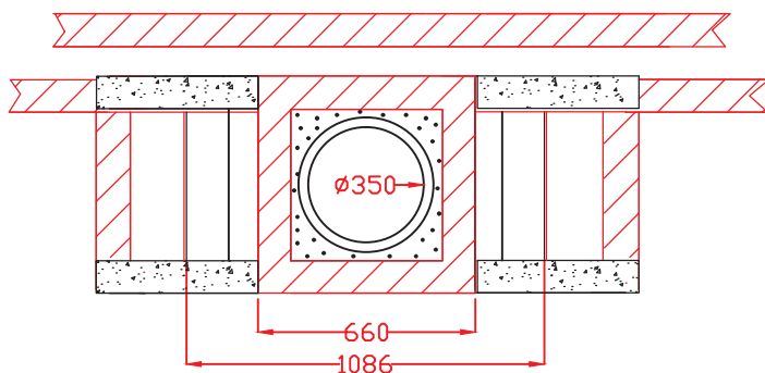
PLAN ABOVE GATHER
