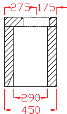
SIDE SECTION OF GATHER
