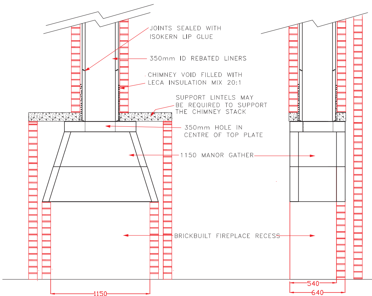
OPTIONAL BACK OFFSET IN LOFT
