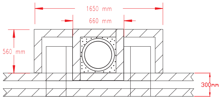
PLAN OF CHIMNEY STACK
